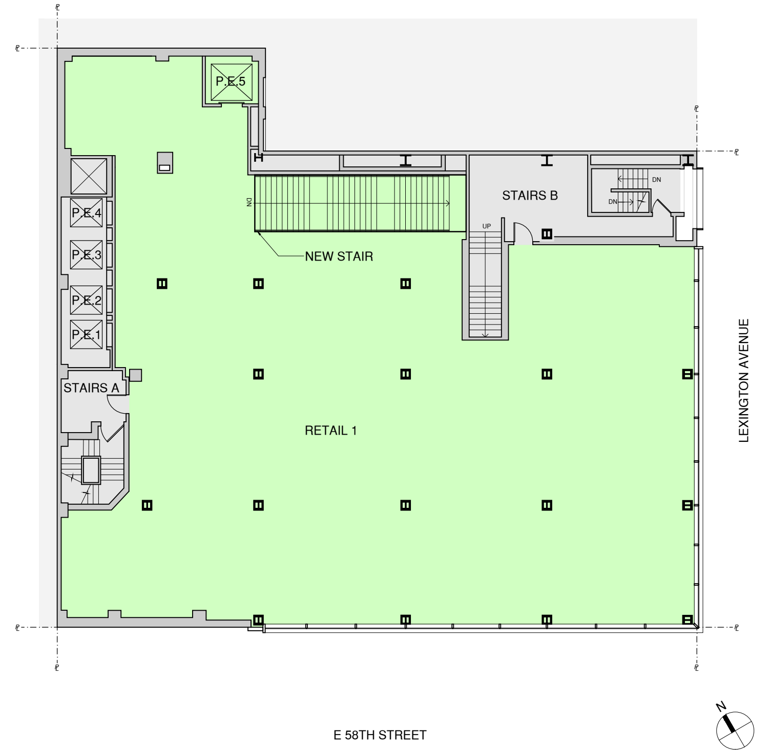
SECOND FLOOR RETAIL 1 7,712 SF
