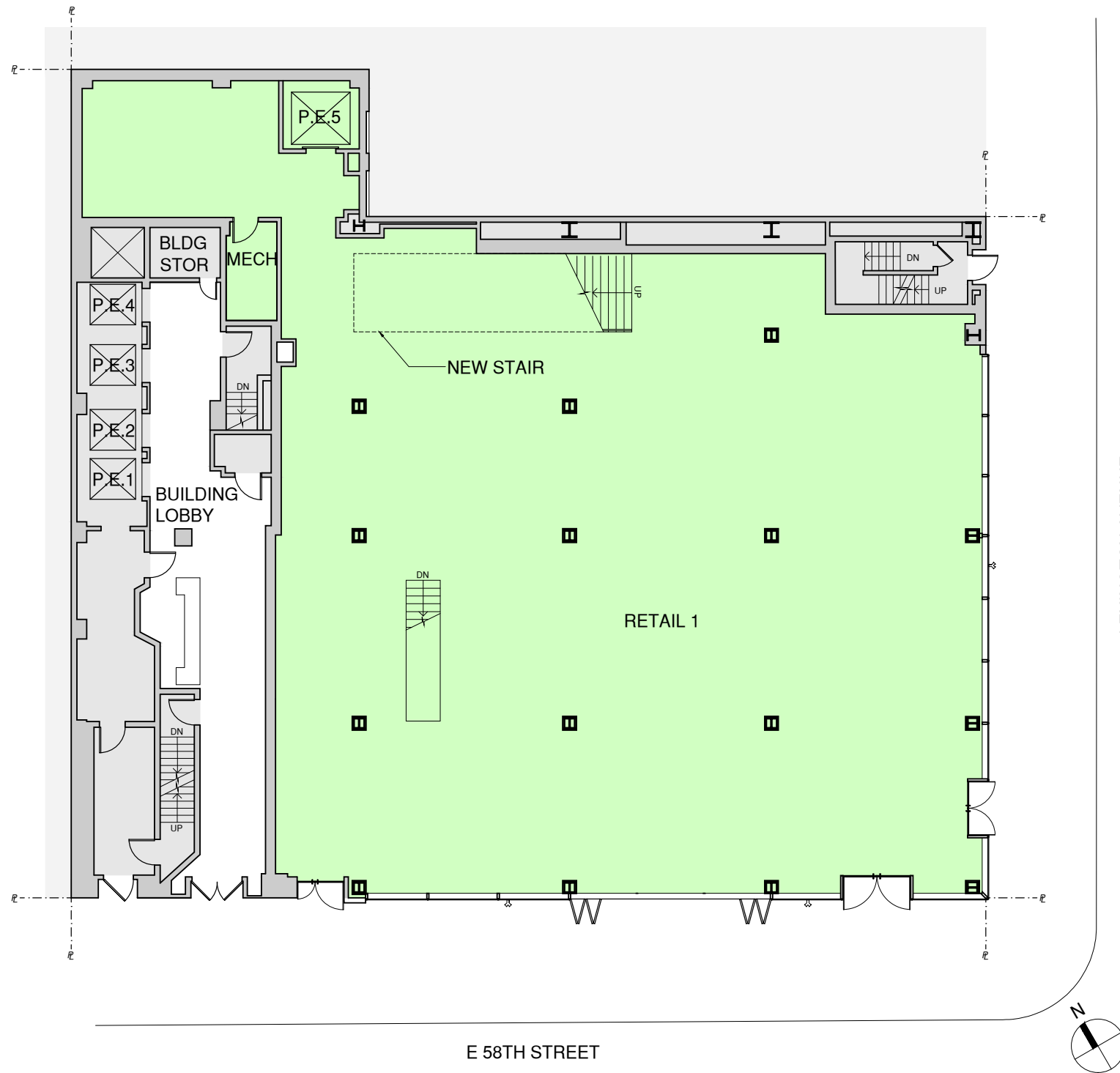
GROUND FLOOR RETAIL 1 7,116 SF
